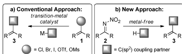
Scheme 1. Nitrimines as alternatives to conventional reagents for metal-free formal C(sp 2 )-C(sp 2 ) cross-coupling chemical reactions. OTf = trifluoromethanesulfonate. OMes = mesylate.
